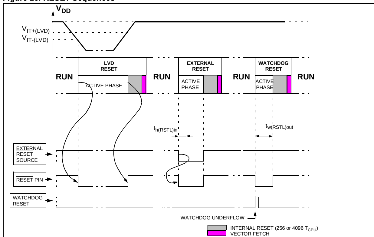
Figure 16. RESET Sequences
