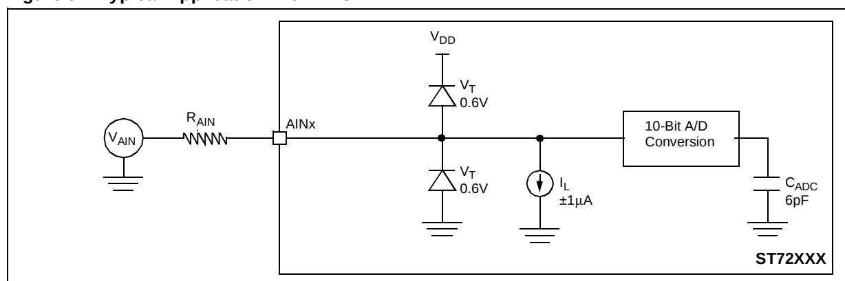
Figure 92. Typical Application with ADC
